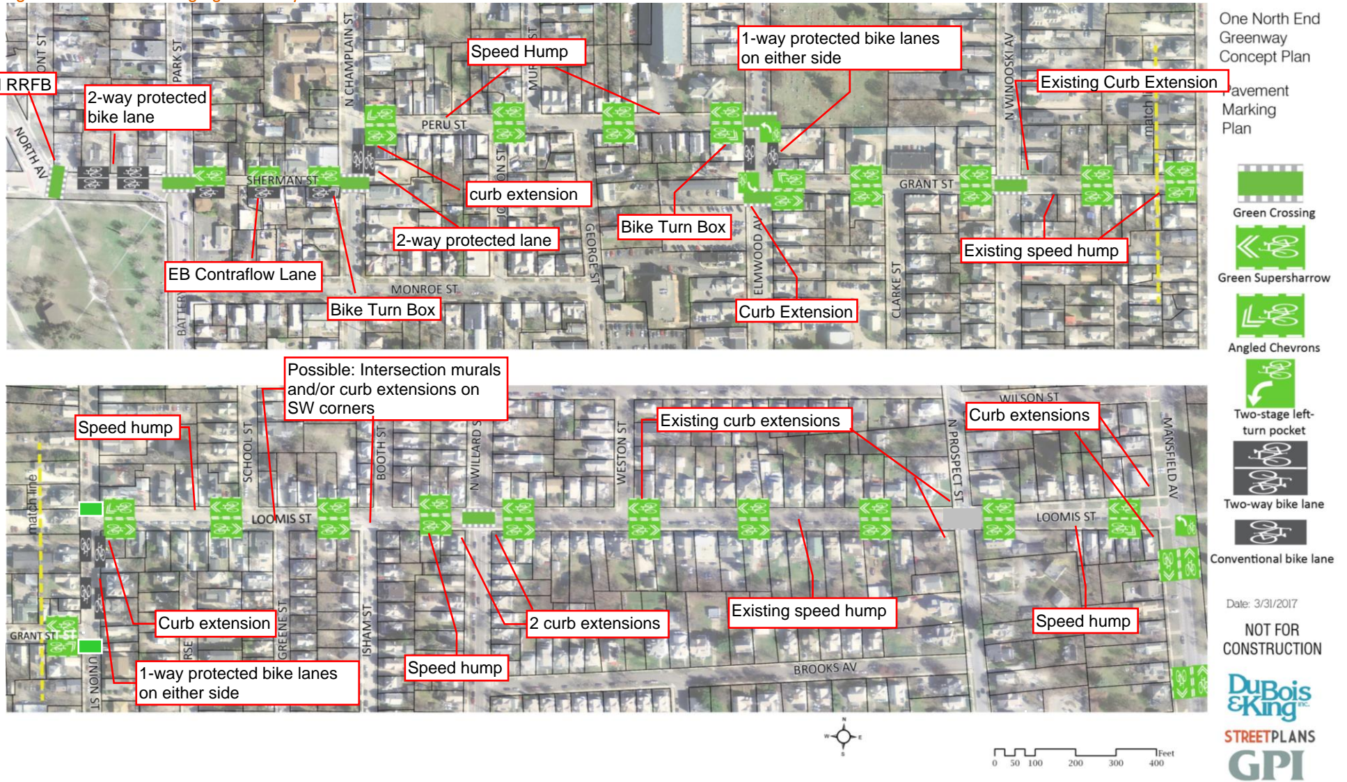
Figure 5.1: Pavement and Signage Greenway Plan
